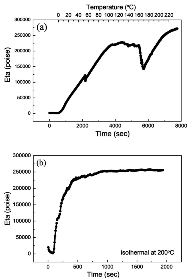
Figure 5. Viscosity of the hybrid low- k films as a function of cure temperature under (a) slow curing profile at 2^{\circ}\text{C}/\text{min} to 250^{\circ}\text{C} and (b) isothermal at 200^{\circ}\text{C} .
